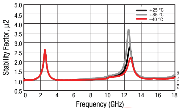
Figure 26. Stability Factor (μ2) vs Frequency and Temperature, Wide Band
