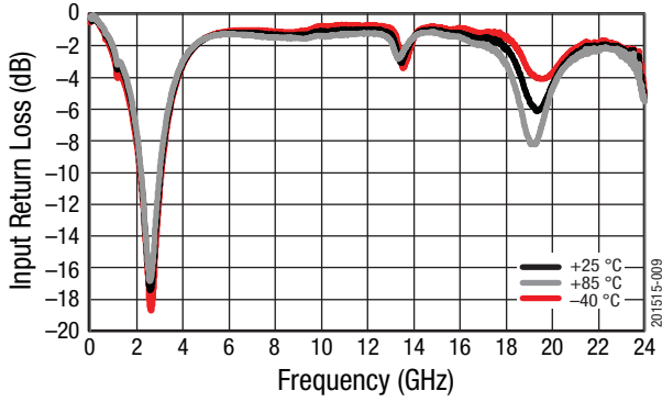
Figure 9. Small Signal Input Return Loss (I S11 I) vs Frequency and Temperature, Wide Band
