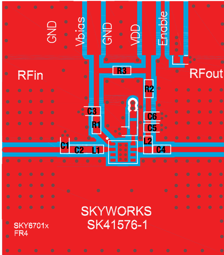
Figure 27. SKY67014-396LF Evaluation Board Assembly Diagram
