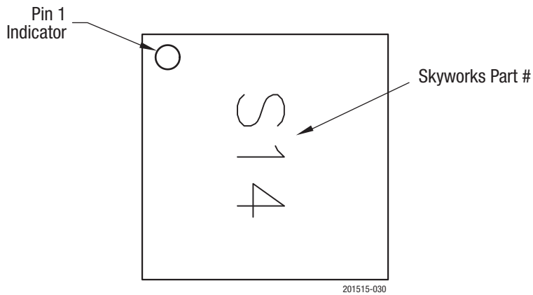
Figure 30. Typical Part Markings (Top View)
