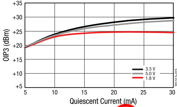
Figure 15. OIP3 vs Quiescent Current and Voltage
