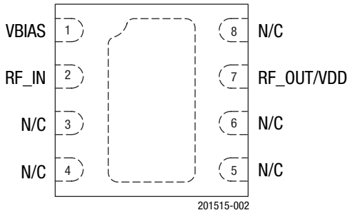
Figure 2. SKY67014-396LF Pinout (Top View)
